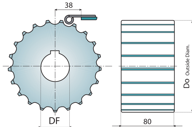
整体式主动轮 (机加工) SINGLE PIECE SPROCKET ( MACHINED )
