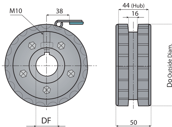
整体式主动轮 (注塑) SINGLE PIECE SPROCKET (INJECTION)
