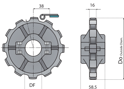
整体式主动轮 (机加工) SINGLE PIECE SPROCKET ( MACHINED )
