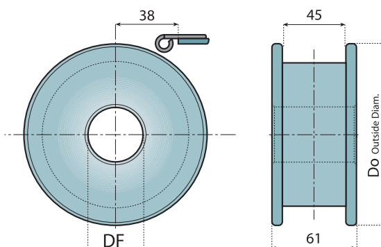
整体式从动轮 (机加工) SINGLE PIECE IDLER WHEEL (MACHINED)
