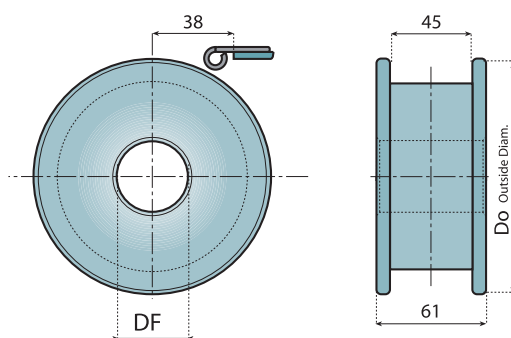
整体式从动轮 (机加工) SINGLE PIECE IDLER WHEEL (MACHINED)
