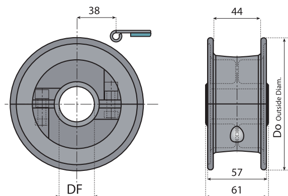
分体式从动轮 (注塑) SPLIT IDLER WHEEL (INJECTION)
