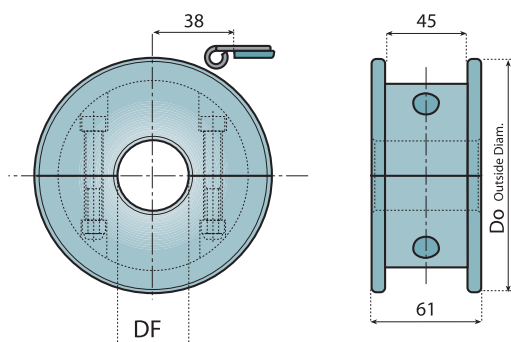
分体式从动轮 (机加工) SPLIT IDLER WHEEL (MACHINED)
