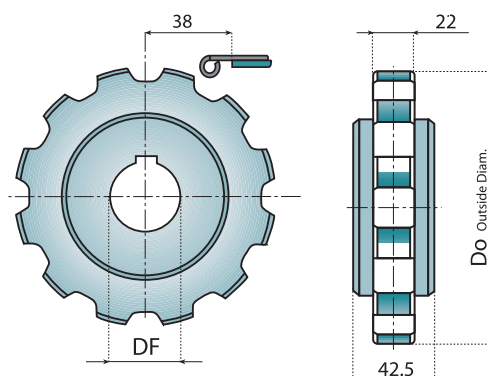
整体式主动轮 (机加工) SINGLE PIECE SPROCKET ( MACHINED )
