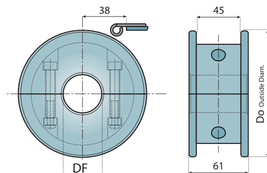
分体式从动轮 (机加工) SPLIT IDLER WHEEL (MACHINED)
